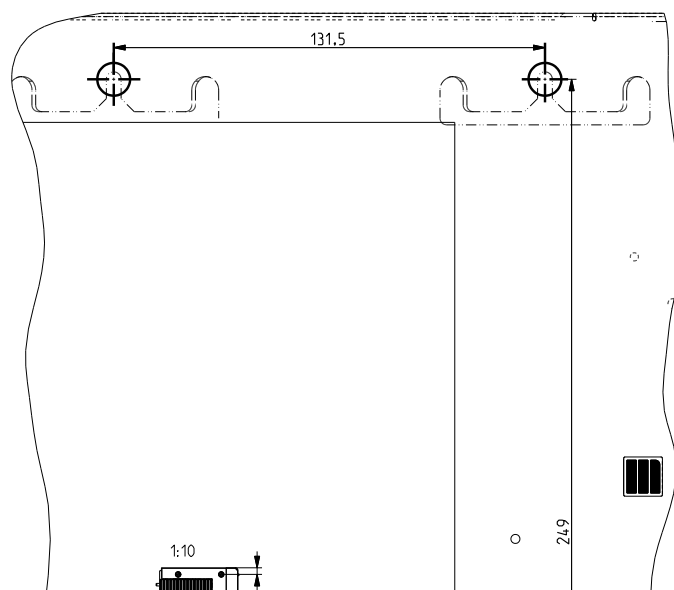
Fig. 2: Dimensions and installation dimensions
