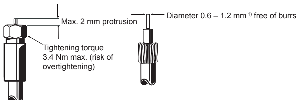
Fig. 3: Attachment of the F-type connector
