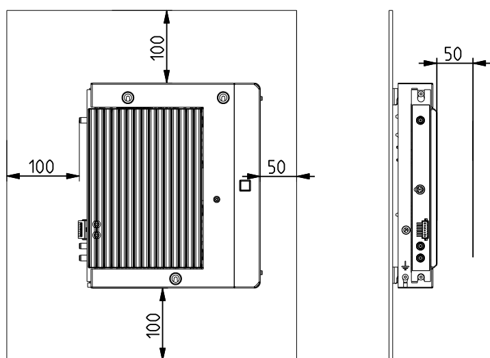
Fig. 1: Clearances to containing surfaces
